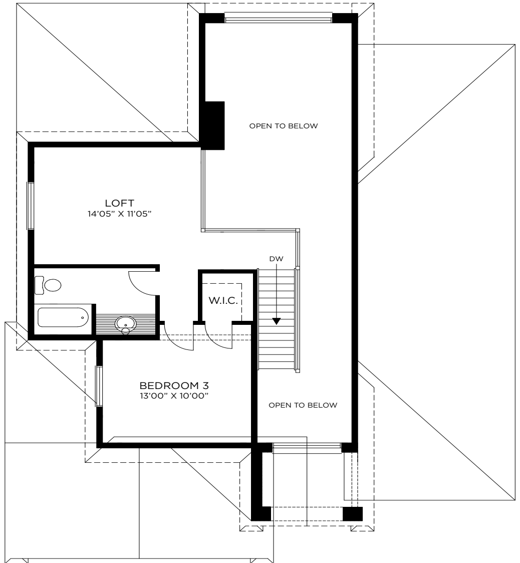
SECOND FLOOR PLAN (OPT. 1)
